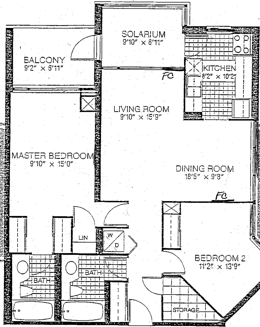
2D SUITES 1/11
